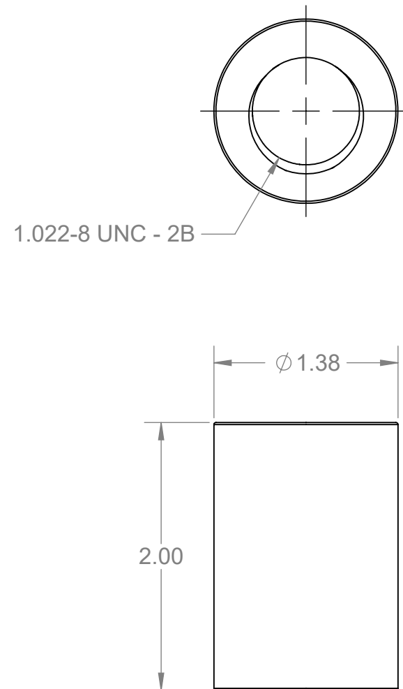
G354 1" AND 3/4" COUPLING NUT
