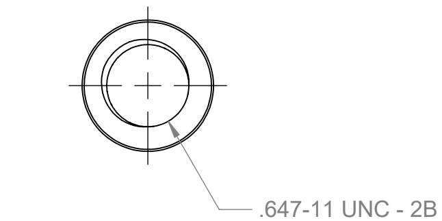
G352 5/8THS COUPLING NUT
